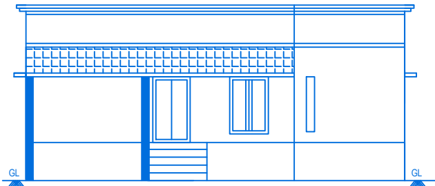
FRONT ELEVATION
