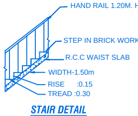
STAIR DETAIL
