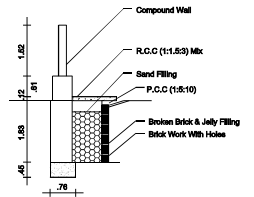
RAIN WATER COLLECTION WELL
