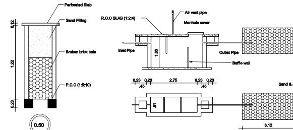
SEPTIC TANK & TRENCH
