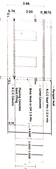
SECTION ON - AA
