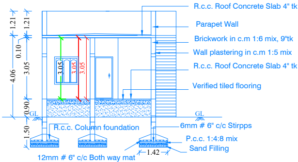
SECTION NN (SCALE: 1CM : 1M)
