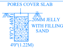
RAINWATER HARVESTING UNIT
