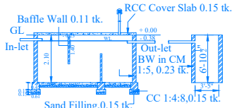
SECTION - SEPTIC TANK
