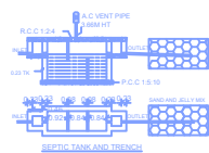
SEPTIC TANK AND TRENCH
