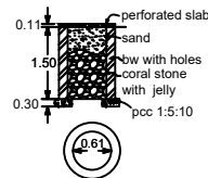
percolation pit
