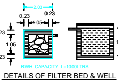
DETAILS OF FILTER BED & WELL
