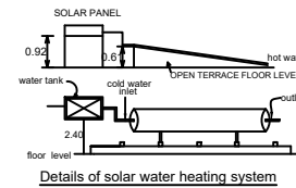
Details of solar water heating system
