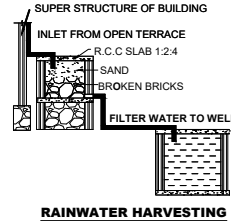
RAINWATER HARVESTING
