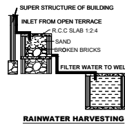
RAINWATER HARVESTING
