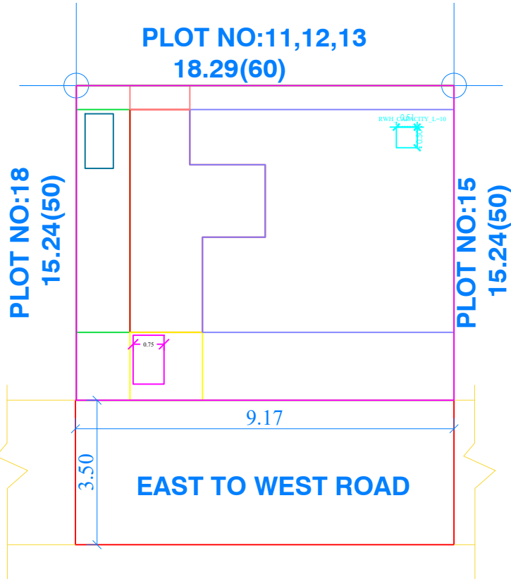
SITE PLAN
