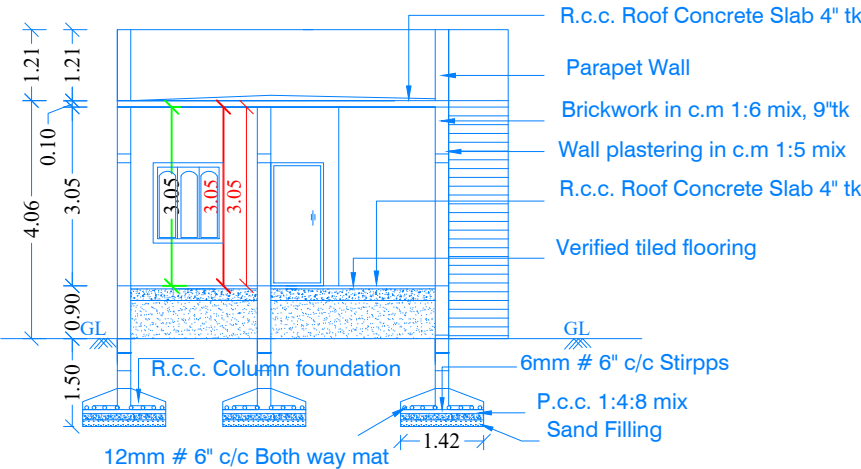
SECTION NN
