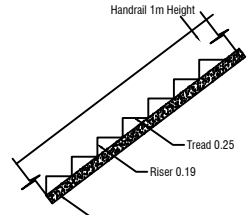
STAIR DETAILS
