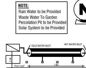
DETAILS OF SOLAR HOT WATER SYSTEM
