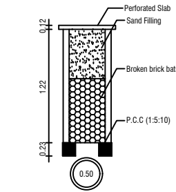
RAIN WATER COLLECTION WELL
