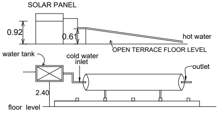
Details of solar water heating system
