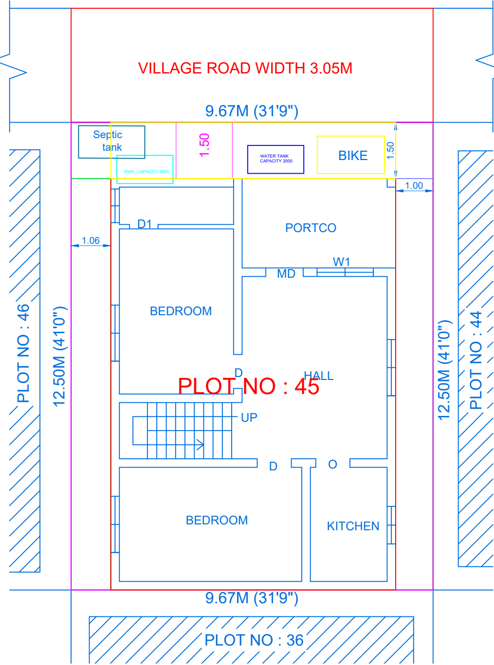
LOCATION PLAN
