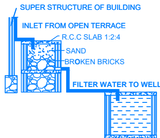
RAINWATER HARVESTING
