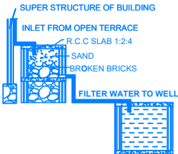
RAINWATER HARVESTING
