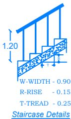
Staircase Details
