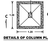
DETAILS OF COLUMN PLAN
