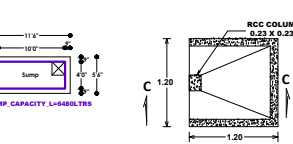
DETAILS OF ECCENTRIC COLUMN PLAN
