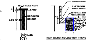
PERCOLATION PIT
