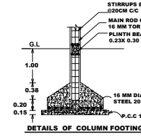
DETAILS OF COLUMN FOOTING
