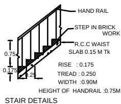
STAIR DETAILS
