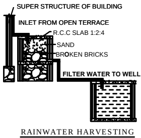
RAINWATER HARVESTING
