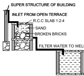
RAINWATER HARVESTING
