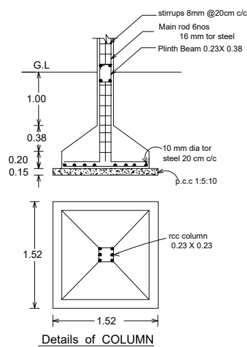
Details of COLUMN
