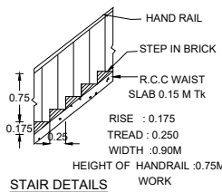
STAIR DETAILS
