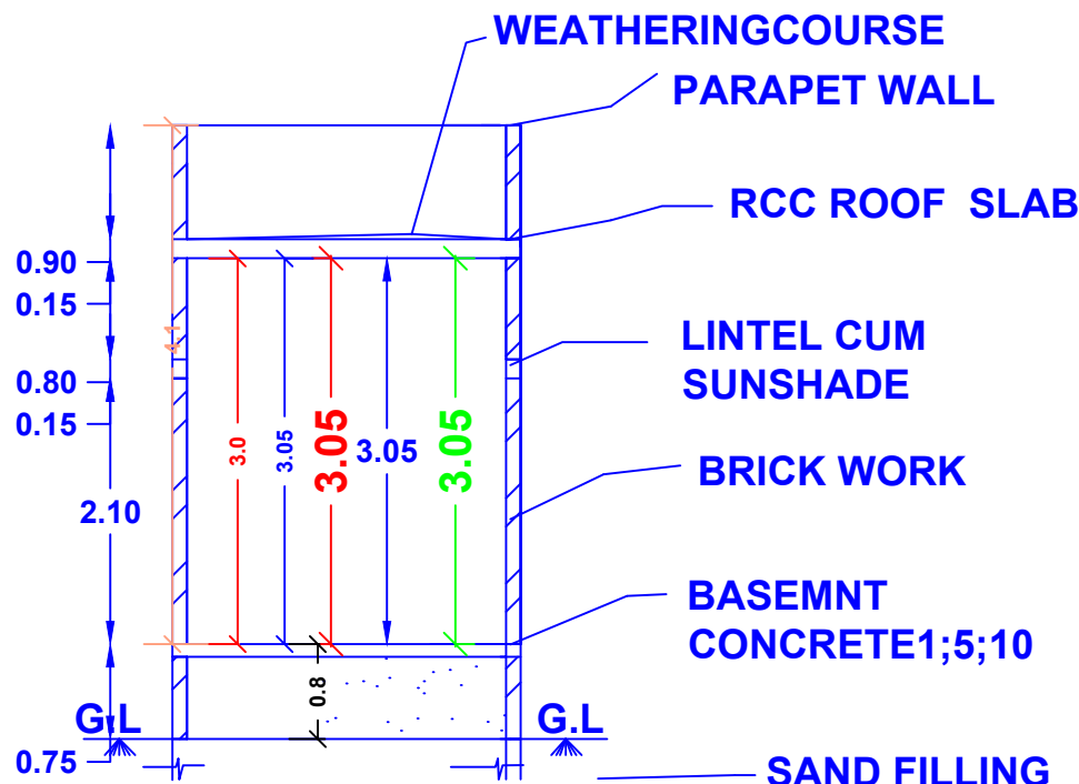
SECTION AB
