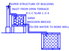
DETAILS OF FILTER BED & WELL
