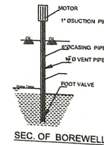
SEC. OF BOREWELL
