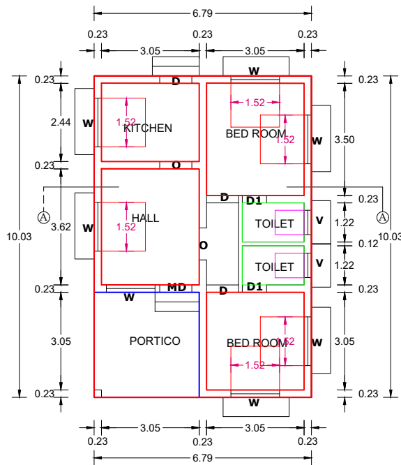
FLOOR PLAN
