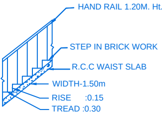
STAIR DETAIL
