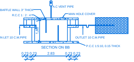
SEPTIC TANK AND TRENCH & U TRAP ADOPTED.
