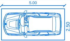
CAR POCKET DETAILS ALL DIMENSIONS ARE IN METRE SCALE 1:100
