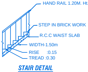
STAIR DETAIL
