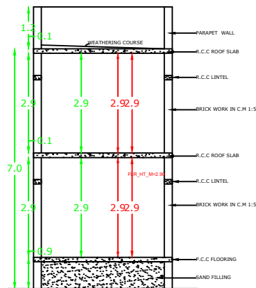
SECTION ON A-A
