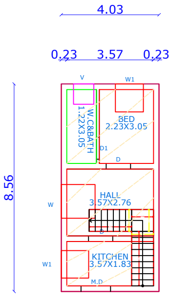
EXG-GROUND FLOOR PLAN
