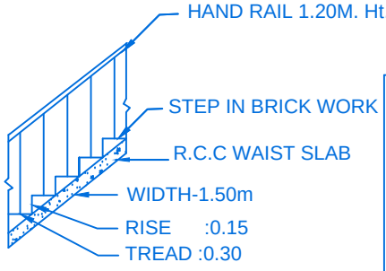
STAIR DETAIL
