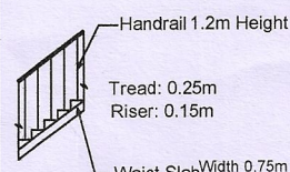
Staircase Details
