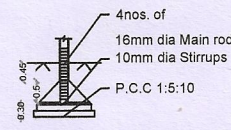
COLUMN FOOTING DETAILS
