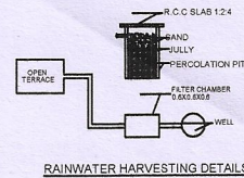
RAINWATER HARVESTING DETAIL:
