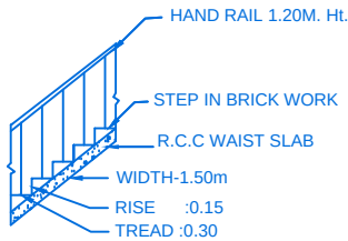
STAIR DETAIL
