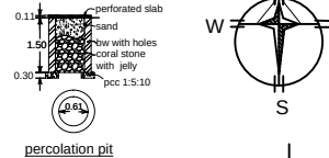
percolation pit
