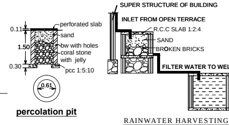
RAINWATER HARVESTING
