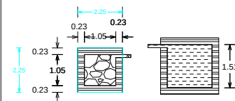
DETAILS OF FILTER BED & WELL
