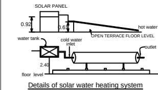
Details of solar water heating system
