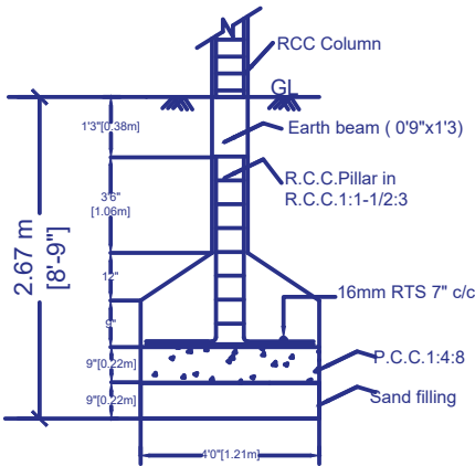
FOUNDATION DETAILS
