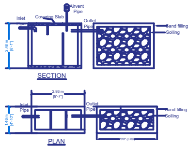
DETAILS OF SEPTIC TANK & DISPERSION TRENCH
