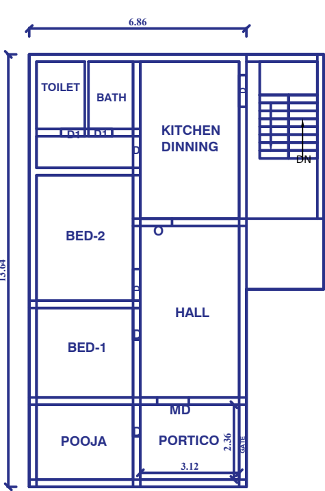
EXIST GROUND FLOOR PLAN
