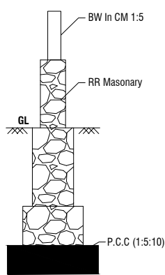
DETAILS OF RR MASONARY
