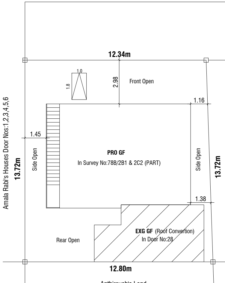
SITE PLAN
