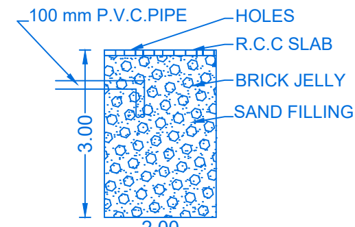
SECTION OF RAIN WATER COLLECTING TANK
