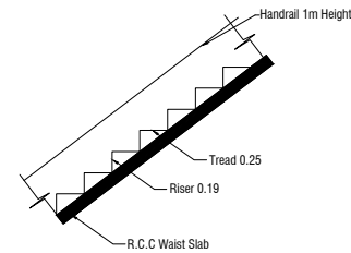
STAIR DETAILS
