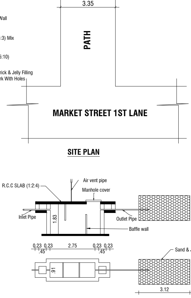
SEPTIC TANK & TRENCH
