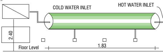
DETAILS OF SOLAR HOT WATER SYSTEM
