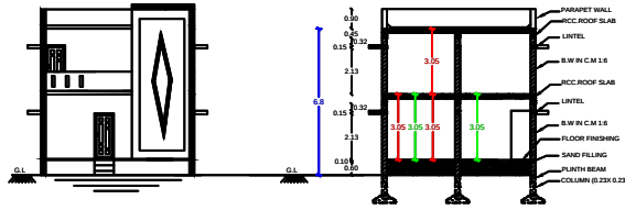
FRONT ELEVATION
