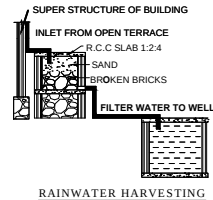
RAINWATER HARVESTING
