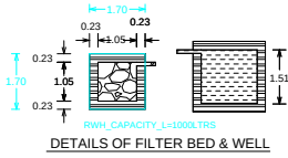
DETAILS OF FILTER BED & WELL
