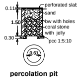
percolation pit
