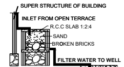
RAINWATER HARVESTING
