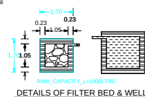
DETAILS OF FILTER BED & WELL
