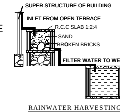
RAINWATER HARVESTING
