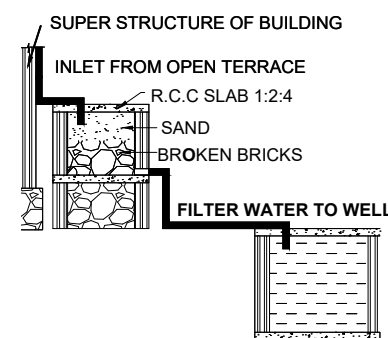
RAINWATER HARVESTING
