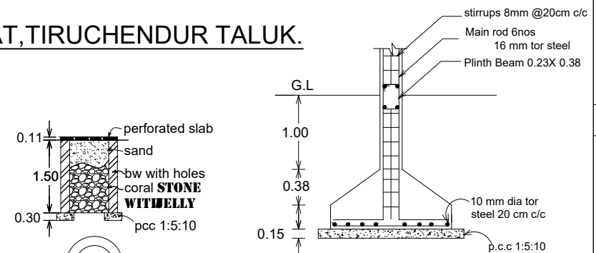
percolation pit
