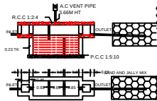
SEPTIC TANK AND TRENCH
