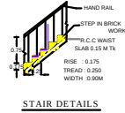
STAIR DETAILS
