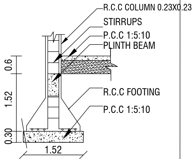
COLOUMN DETAILS
