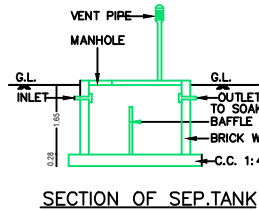
SECTION OF SEP.TANK
