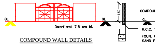
COMPOUND WALL DETAILS
