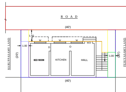
SITE PLAN (SCALE :- 1:100)
