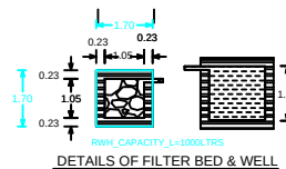
DETAILS OF FILTER BED & WELL
