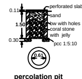
percolation pit
