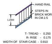
DETAILS OF STAIRCASE
