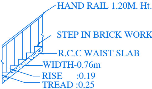
STAIR DETAIL
