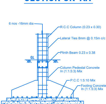
COLUMN FOOTING DETAILS
