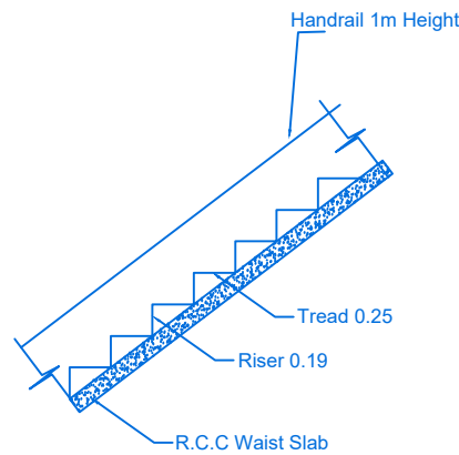
STAIR DETAILS
