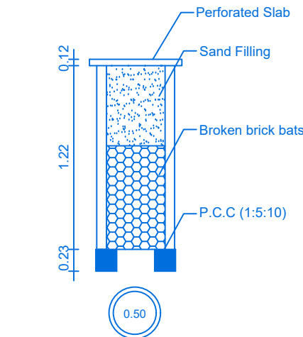
RAIN WATER COLLECTION WELL
