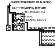
RAINWATER HARVESTING
