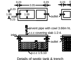
Details of septic tank & trench
