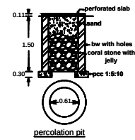
percolation pit
