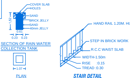
STAIR DETAIL
