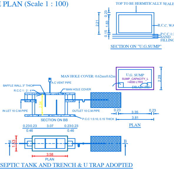
SEPTIC TANK AND TRENCH & U TRAP ADOPTED
