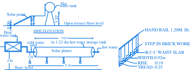
STAIR DETAIL
